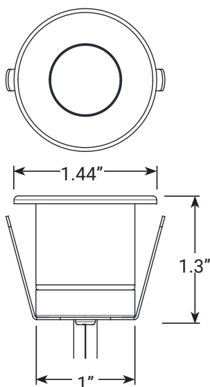
Fixture Body
