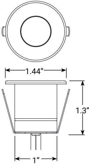
Fixture Body
