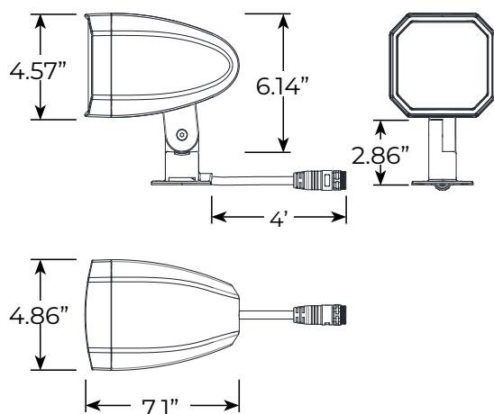
SATELLITE SPEAKER
