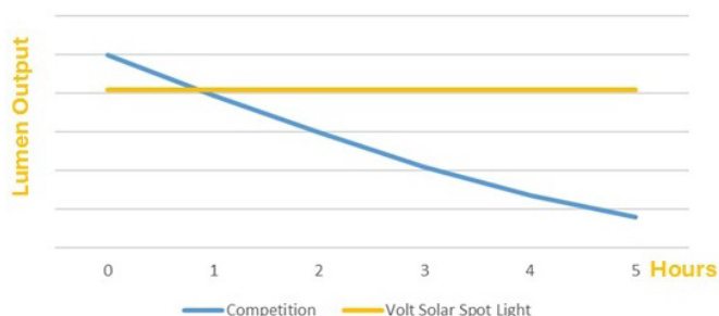
Lumen Output Over Time VOLT Solar Spotlight
